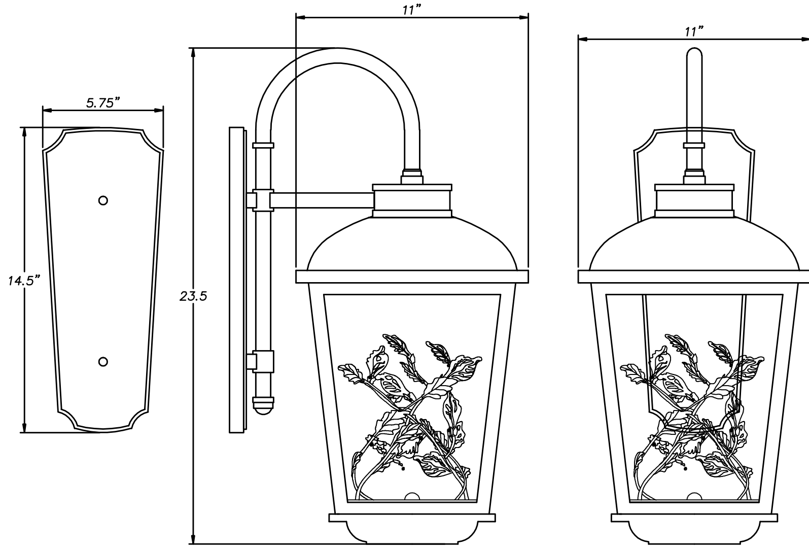
Fixture
