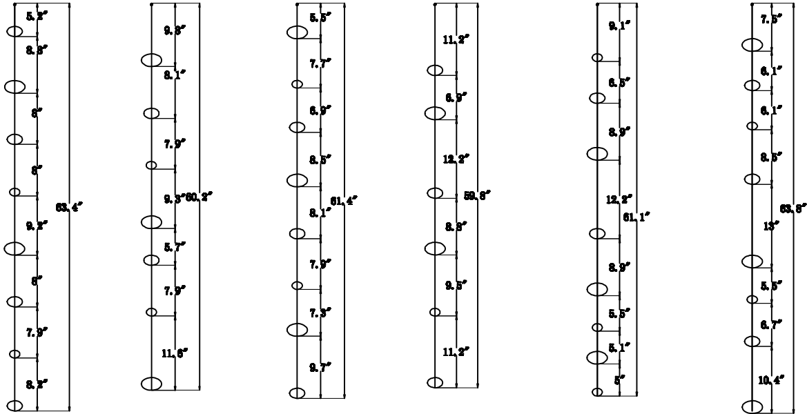
CRS39855PCA*1PC L:63.39" CRS39855PCB*1PC L:60.24" CRS39855PCC*1PC L:61.42" CRS39855PCD*2PCS L:59.84" CRS39855PCE*2PCS L:61.02" CRS39855PCF*2PCS L:63.78"
