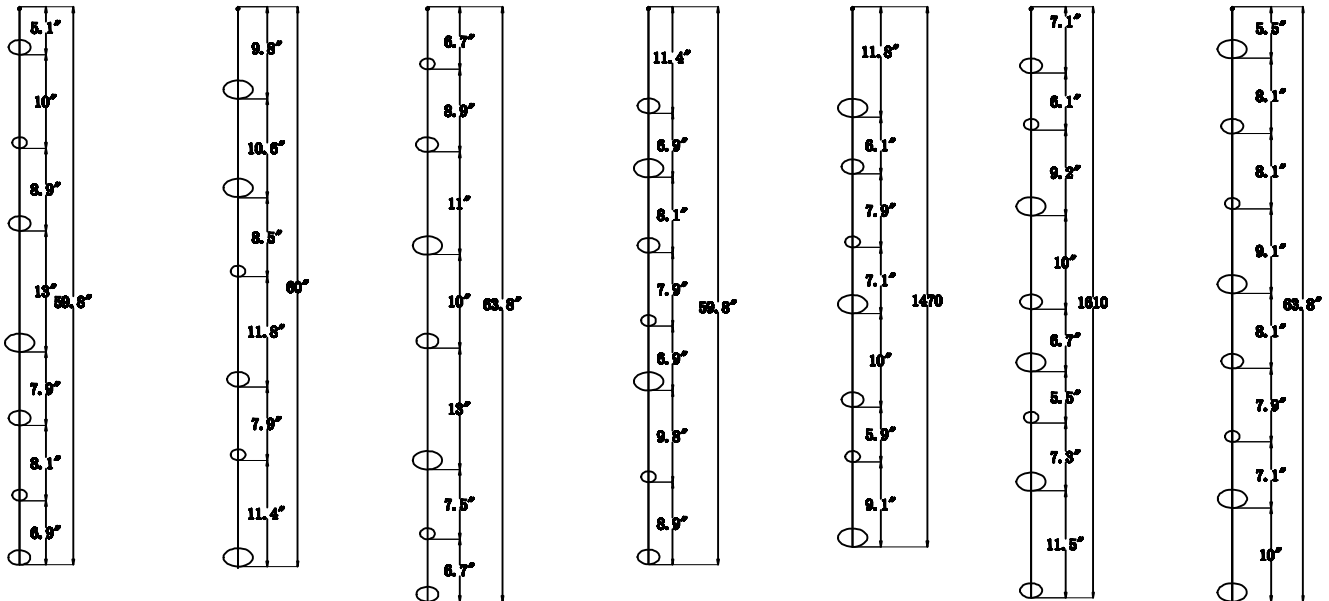
CRS39855PCG*2PCS L:59.84" CRS39855PCH*1PC L:60.04" CRS39855PCI*1PC L:63.78" CRS39855PCJ*1PC L:59.84" CRS39855PCK*1PC L:57.87" CRS39855PCL*1PC L:63.39" CRS39855PCN*1PC L:63.78"
