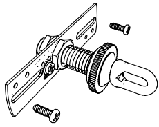
Mounting Strap (A)
