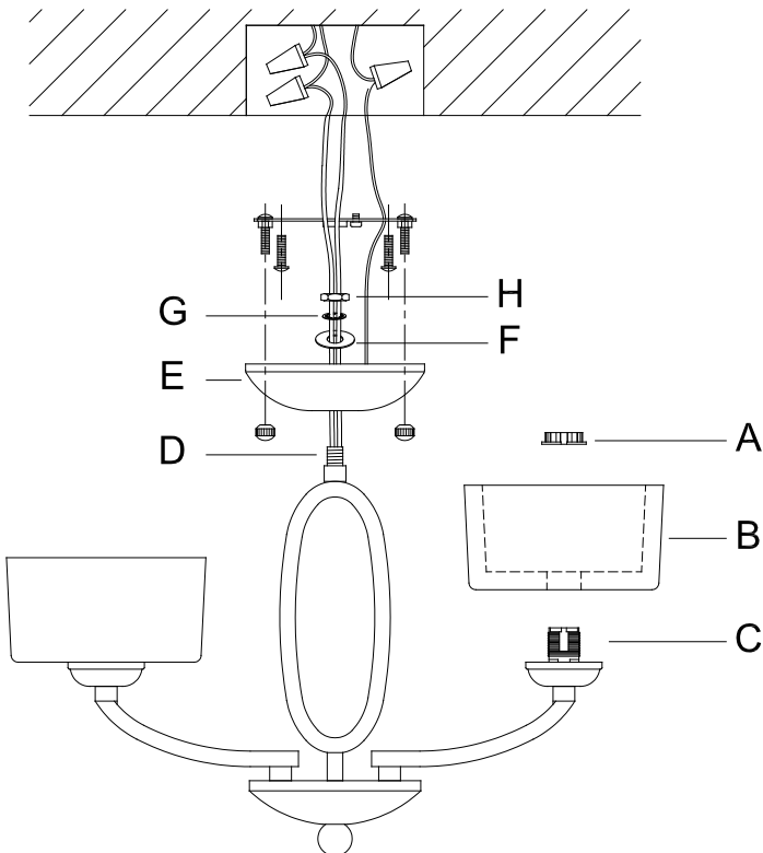
Semi-Flush Mount
